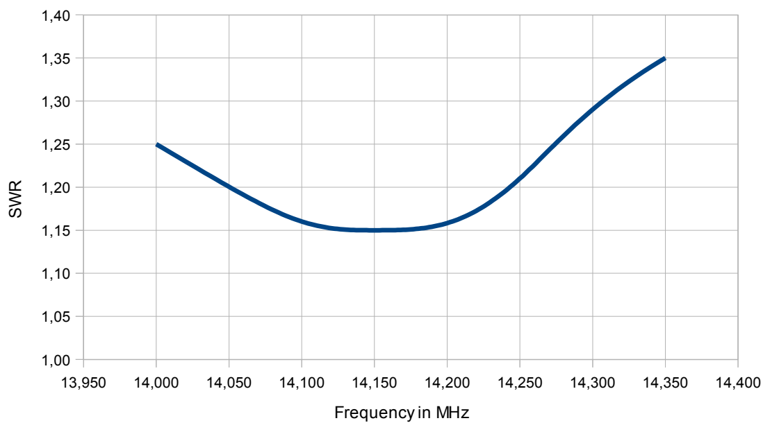
SWR measured with Revex W570
