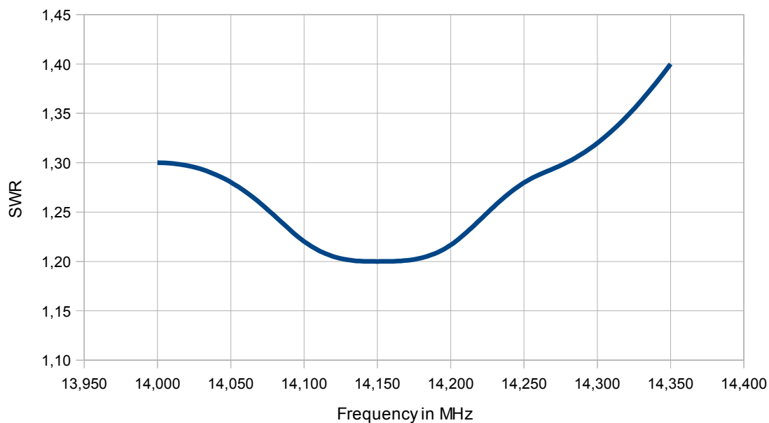
SWR measured with MFJ-259B
